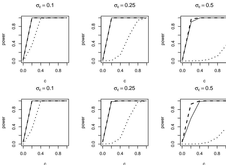
Figure 1: Power curves of three testing procedures
